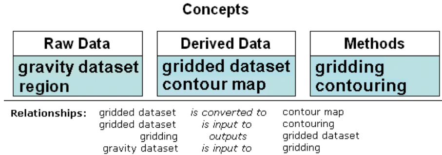
Fig. 1. Gravity Ontology.
